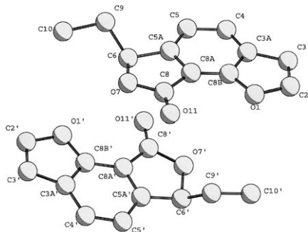
Fig. 2. X-Ray stereo drawing of concentricolide ( 1 )
